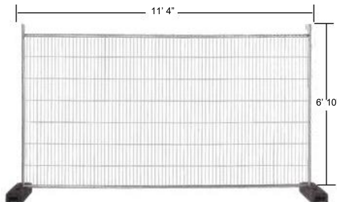
Welded wire grid 1-1/2" x 10-1/2"
